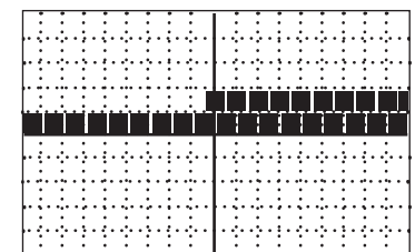
Perpendicular Grid with 1st Row placement and 2nd row beginning brick pattern.
