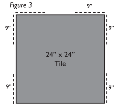
Tile to Tile CX-948 Placement 1/4" wide bead 9" in from all 4 edges.
